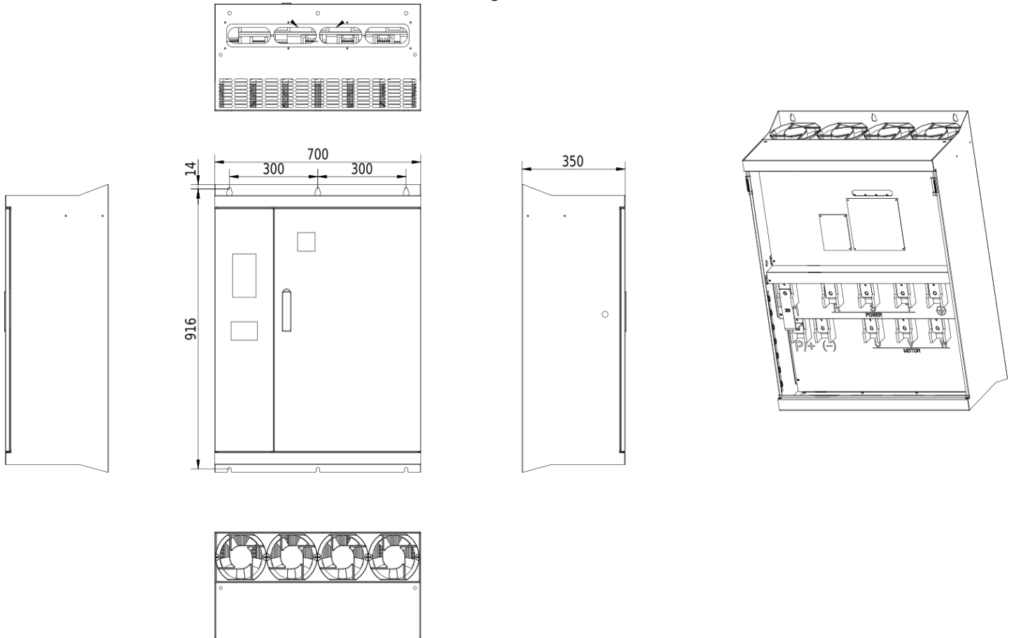
Dimensional drawing V810 - 315kW 4T3150
