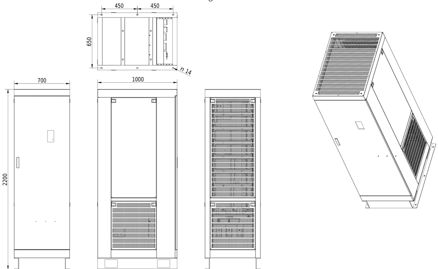
Dimensional drawing V810 - 800kW 4T8000
