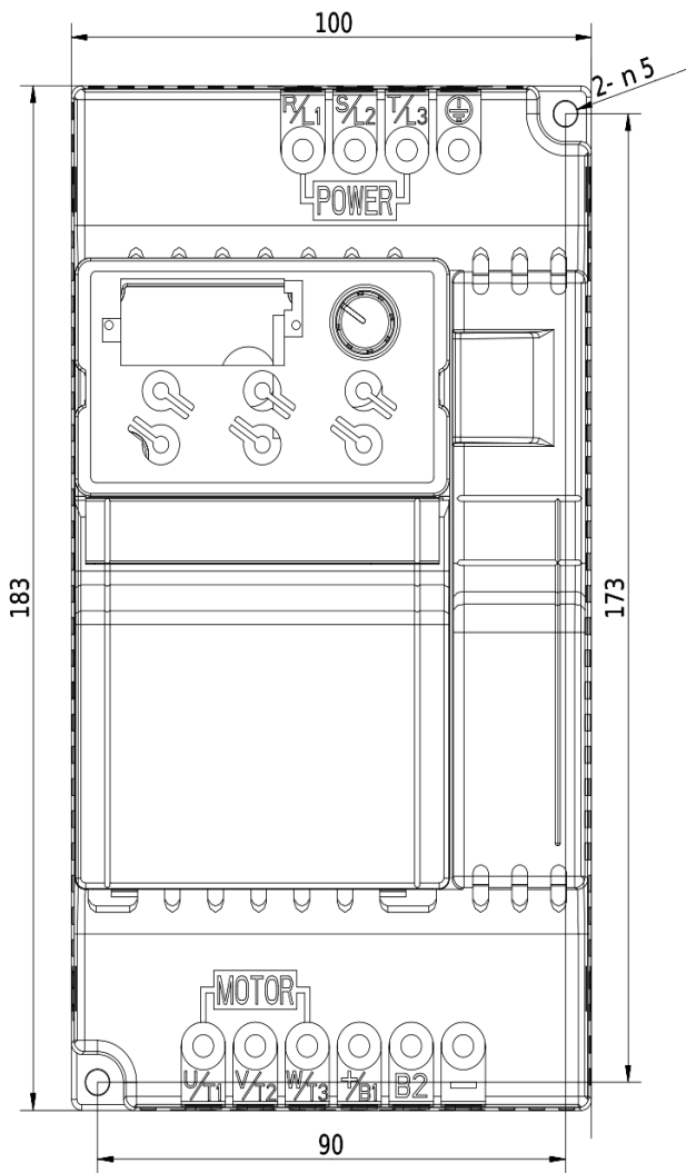
Dimensional drawing V800 - 2,2kW 2S0022
