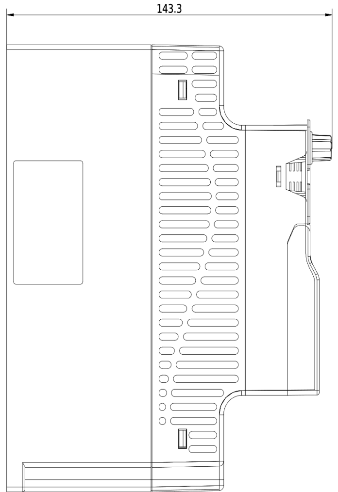
Dimensional drawing V800 - 2,2kW 2S0022
